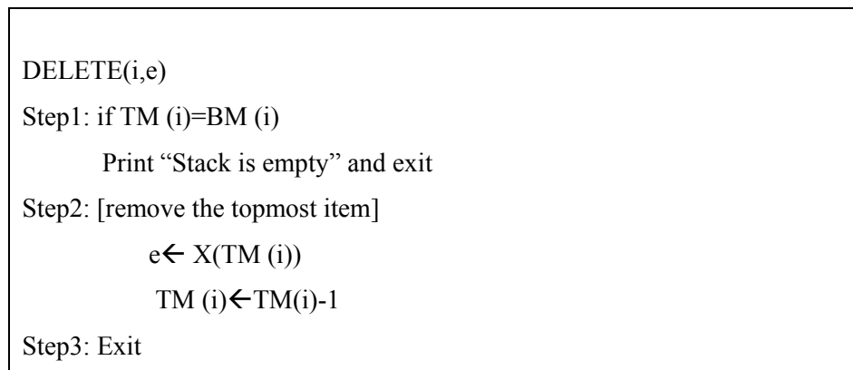
Figure 4.7: Algorithm to delete an element from i^{\text{th}} stack
