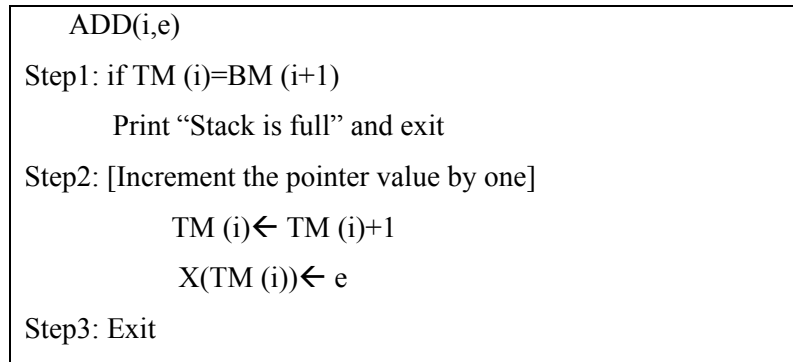
Figure 4.6: Algorithm to add an element to i^{\text{th}} stack
