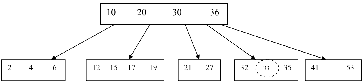
Figure 7.12 : A B-tree
