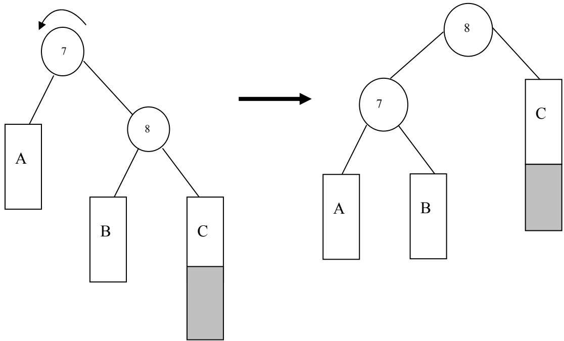
Figure 7.9: LL Rotation
