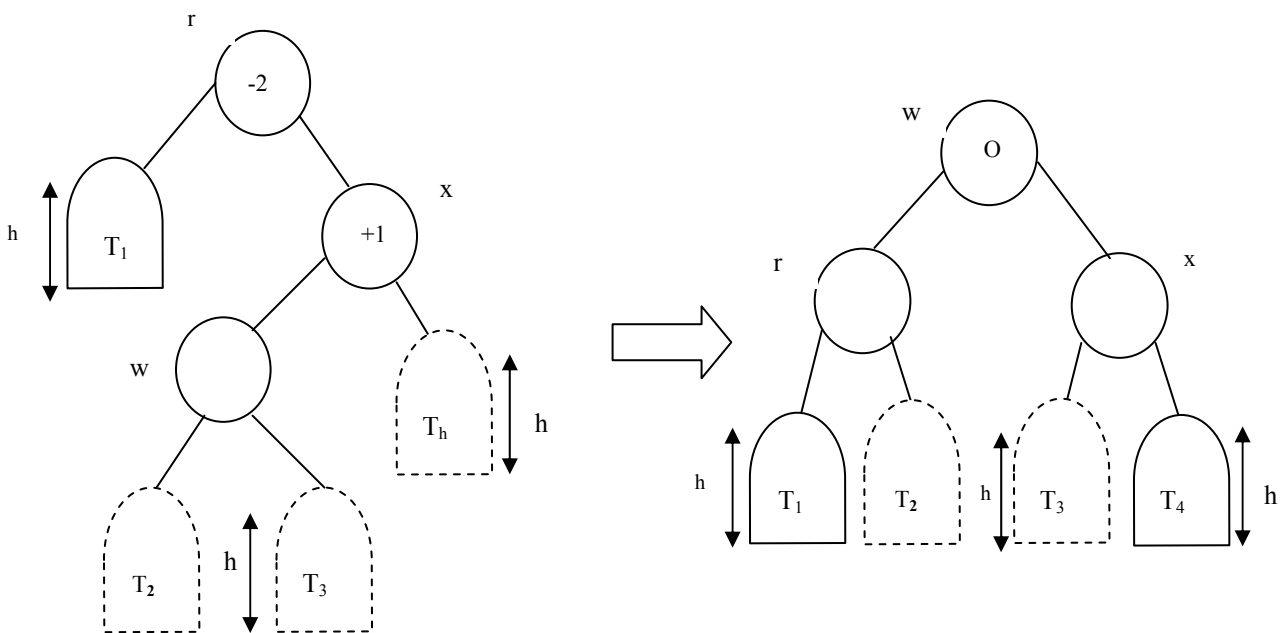
Figure 7.8: RL Rotation
